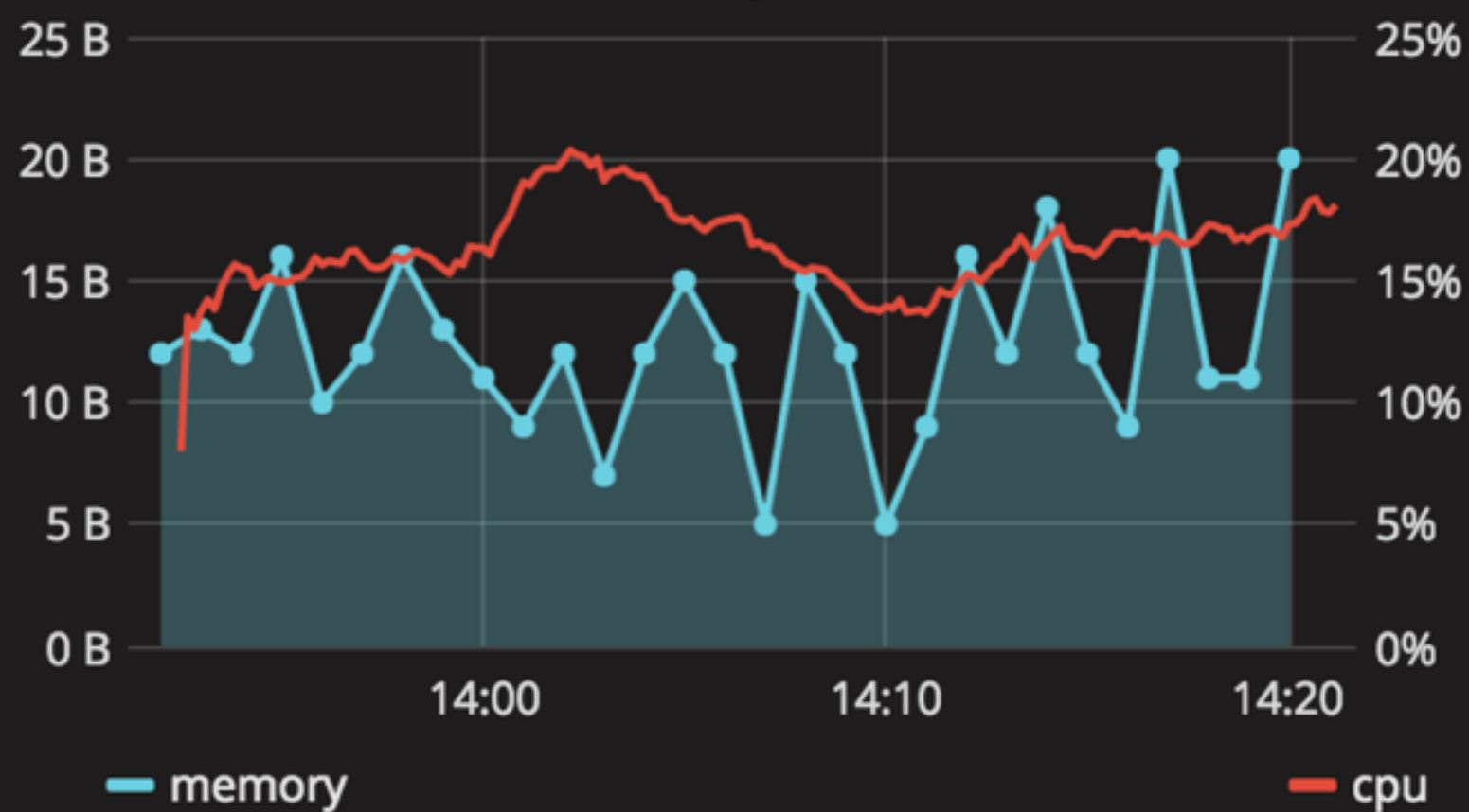
Memory / CPU
