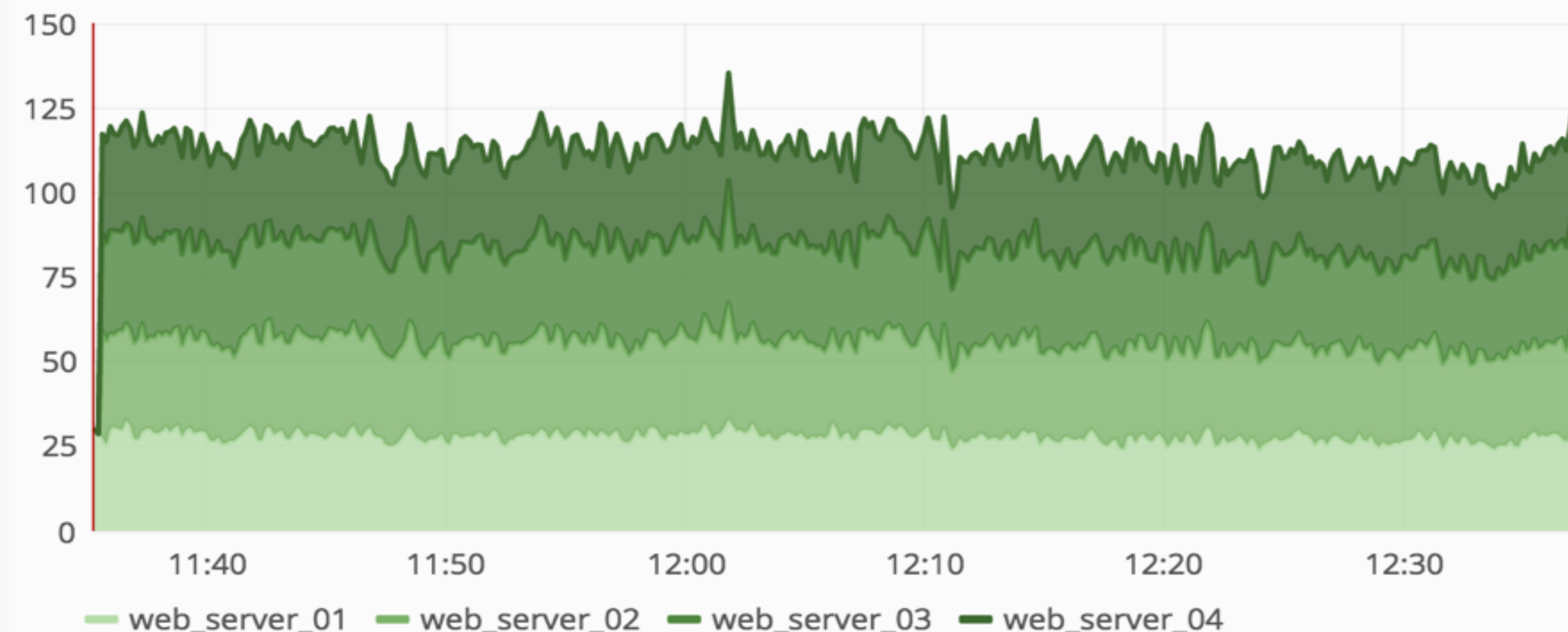
server requests
