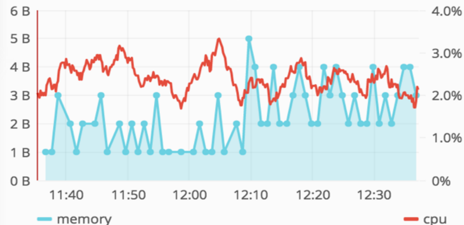
Memory / CPU
