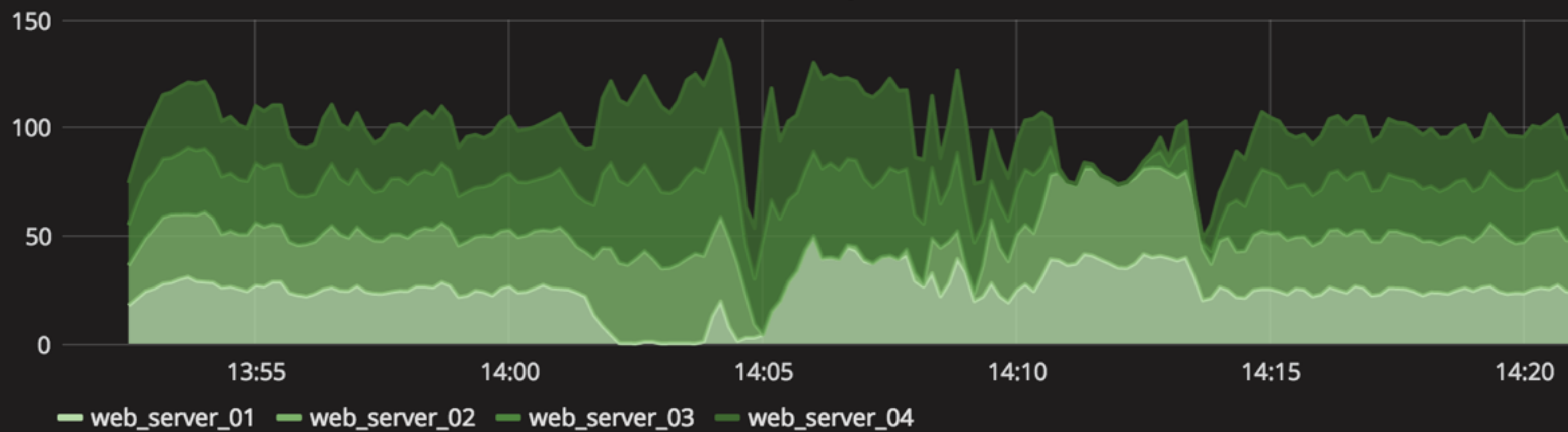
server requests
