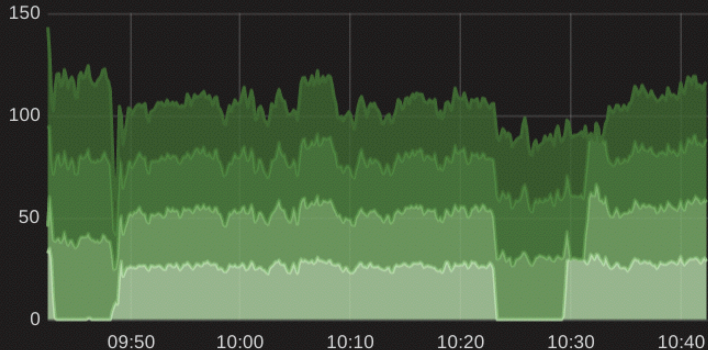
server requests
